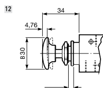
Knopf – G1/8-Ventile
