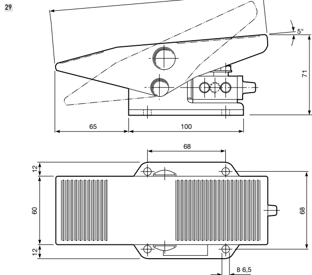
Hebel/Feder/Hebel - G1/4-Ventile
