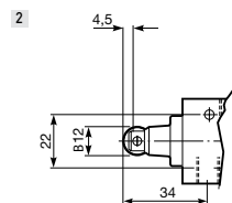
Rolle – G1/4-Ventile
