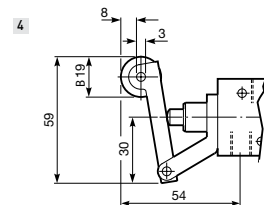
Tastrolle – G1/8-Ventile
