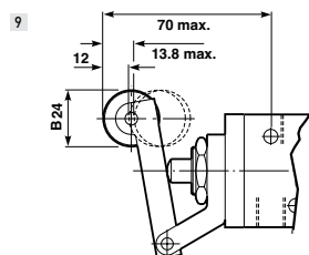
Tastrolle – G1/4-Ventile
