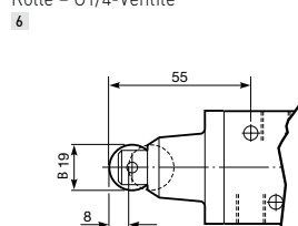
Rolle – G1/4-Ventile
