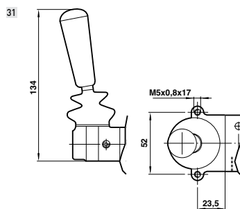
Hebel - G1/4-Ventile
