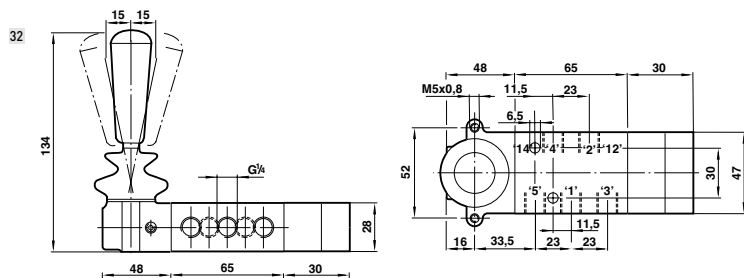
Hebel/Feder/Hebel - G1/4-Ventile
