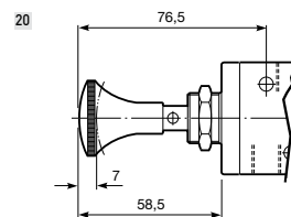
Knopf – G1/4-Ventile
