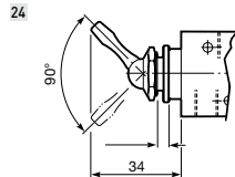
Schlüssel - G1/8-Ventile
