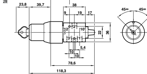
Hebel - G1/4-Ventile
